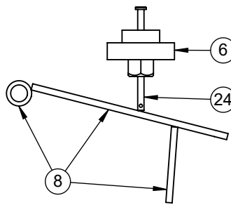
Detail A Scrap Ejector Assembly
