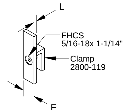
Leaf Finger Includes leaf finger, clamp, bolt
