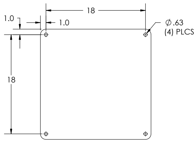
MOUNTING PATTERN
