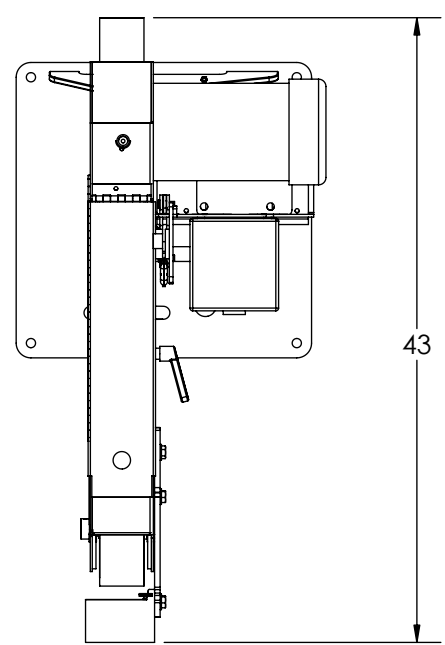
TOP VIEW
