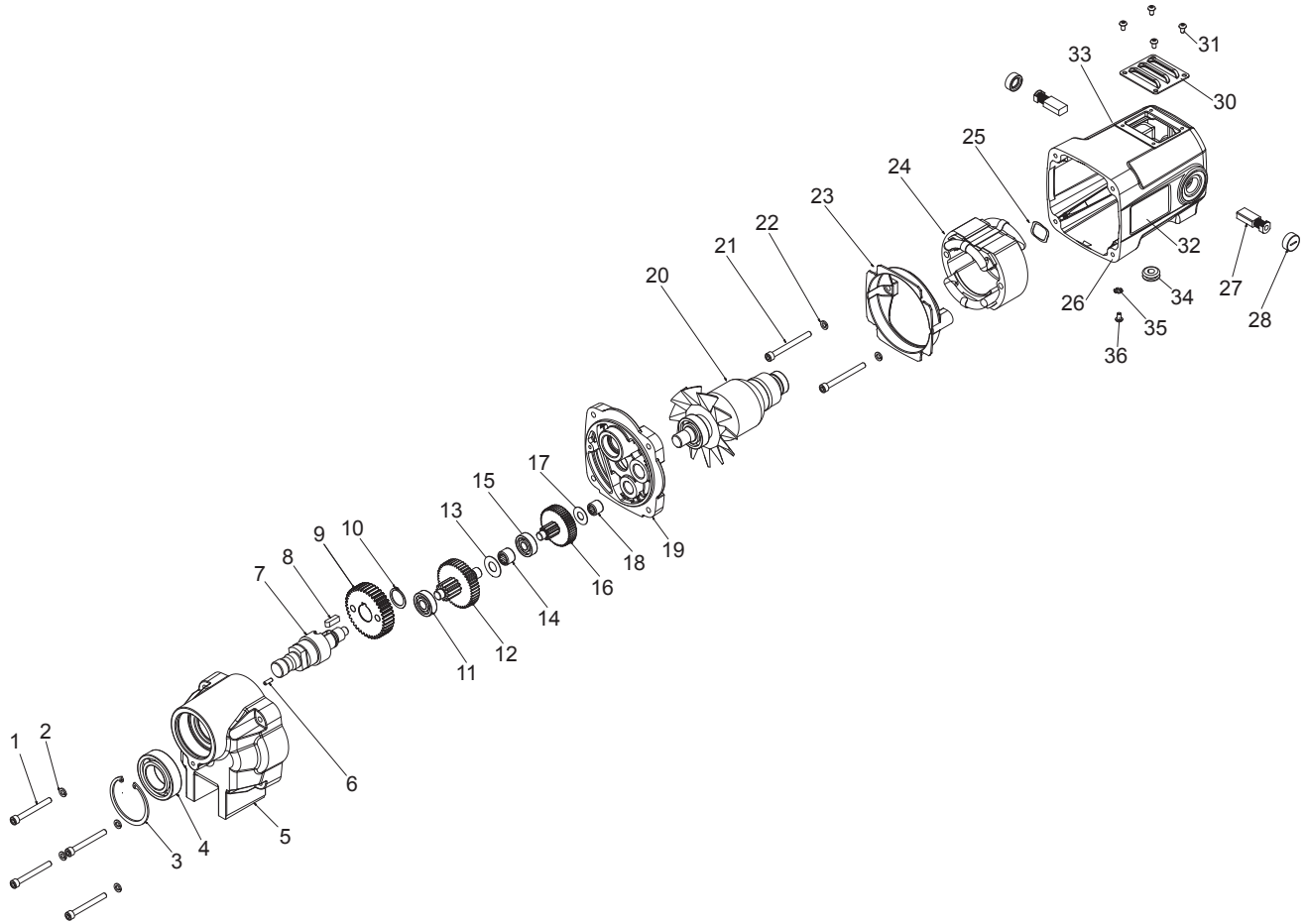
09134 Motor Assembly
