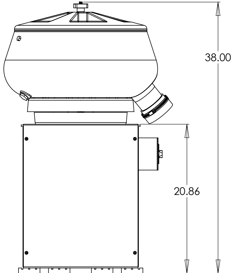
BACK VIEW
